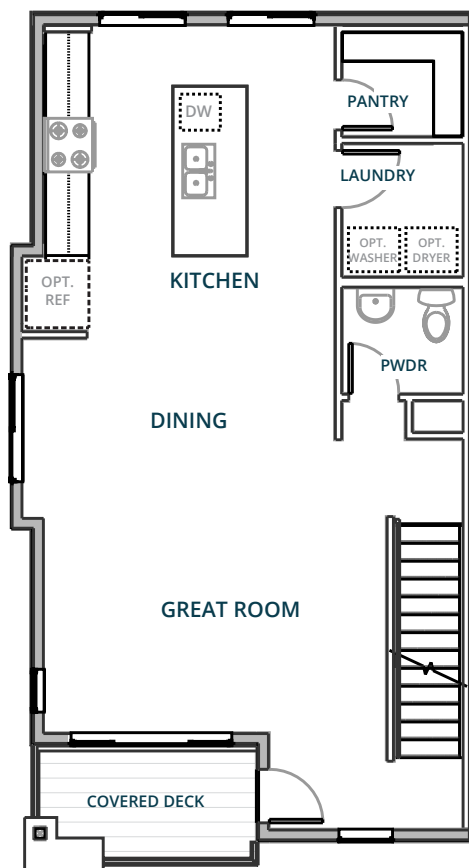
MAIN FLOOR
